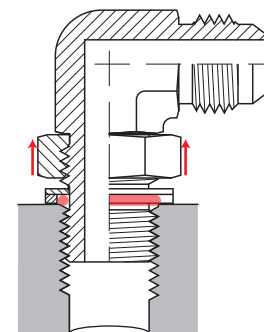
Adjustable nut and washer are backed all the way off. Fitting is threaded in until seal is touching the port. Fitting is not oriented yet.
