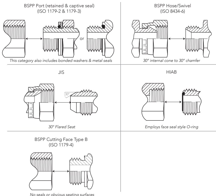
BSPP Threads and Sealing Methods
