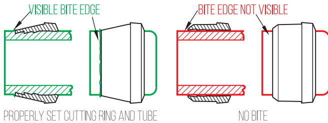
PROPERLY SET CUTTING RING AND TUBE
